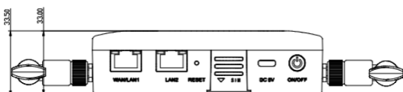
Interface Dimensions
