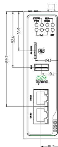
Interface Diagram
